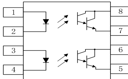
Pin Configuration
