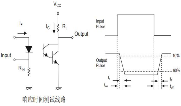
Fig.7 Switching Time Test Circuit & Wave forms
